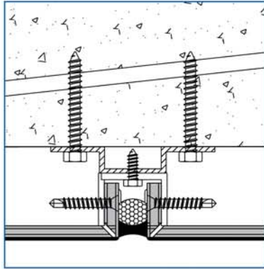
Wet-Seal System
